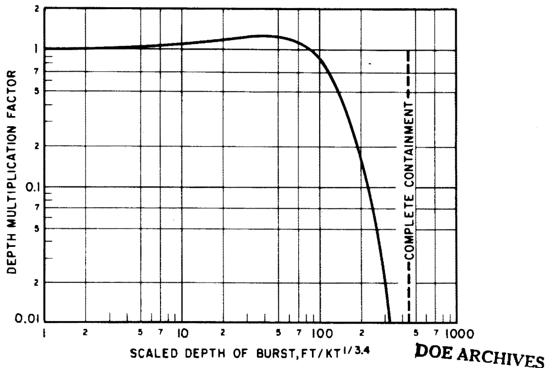
Figure 4-45. Depth Multiplication Factor for Linear Contour Dimensions vs. Scaled Depth of Burst
